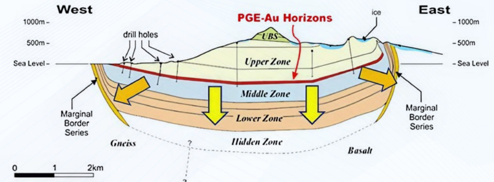
East-West Geological Section (Looking North)
